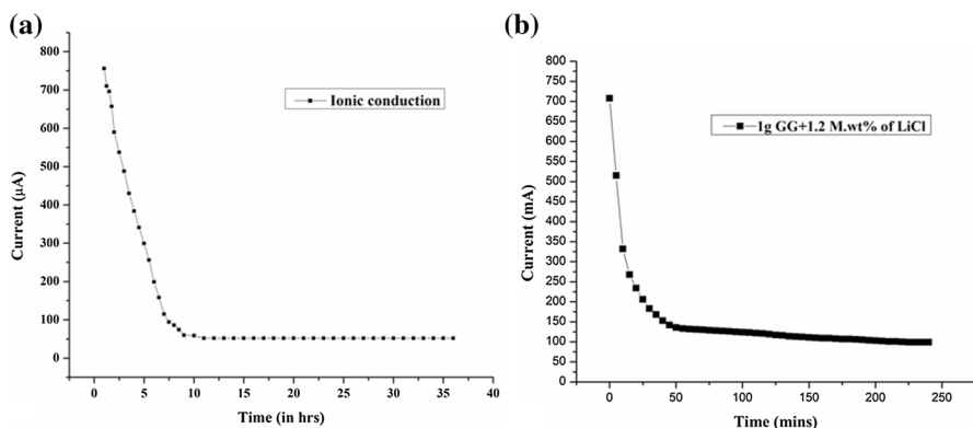
Fig. 7 a Variation in DC current with respect to time and b current versus time plot for high ion conducting membrane of 1 g GG + 1.2 M wt% of LiCl
